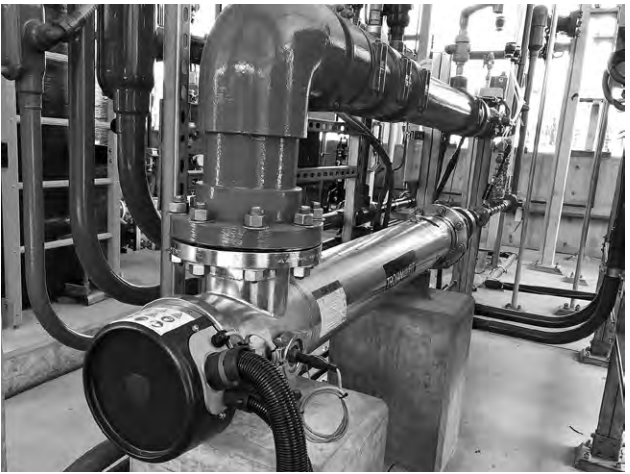
A view of the Regional Recycled Water Program demonstration facility.
